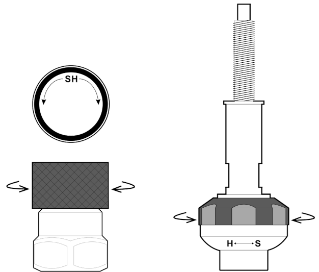
FRONT KNOB
